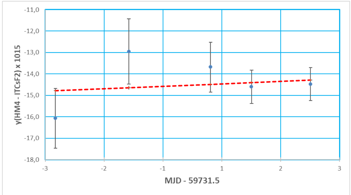
Figure 3. y(HM4 - ITCsF2) data and the linear fit curve centered in MJD 59731.5
