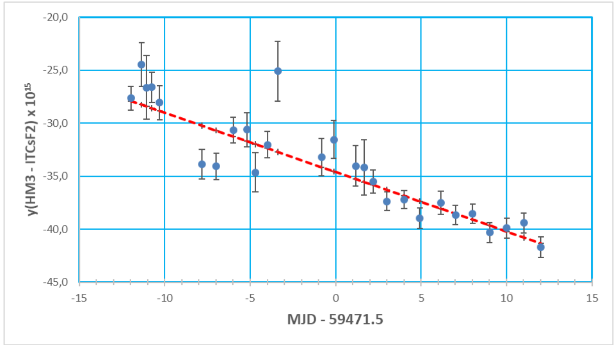
Figure 3. y(HM3-ITCsF2) data and the linear fit curve centered in MJD 59471.5
