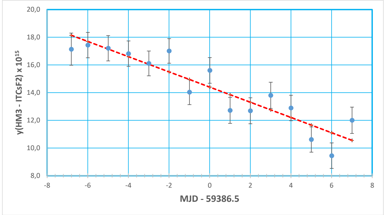
Figure 3. y(HM3-ITCsF2) data and the linear fit curve centered in MJD 59386.5
