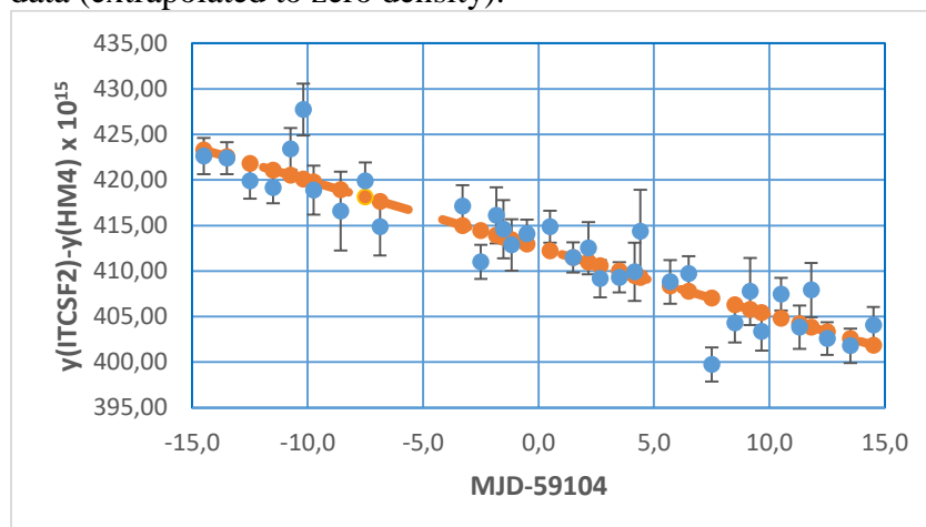
Figure 3. y(ITCsF2) - y(HM4) data and the linear fit curve centered in MJD 59104.
