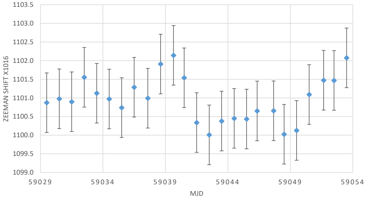
Figure 1. Zeeman shift fluctuations during the TAI evaluation period.
