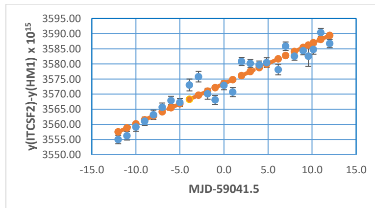
Figure 3. y(ITCsF2) - y(HM1) data and the linear fit curve centered in 59041.5.
