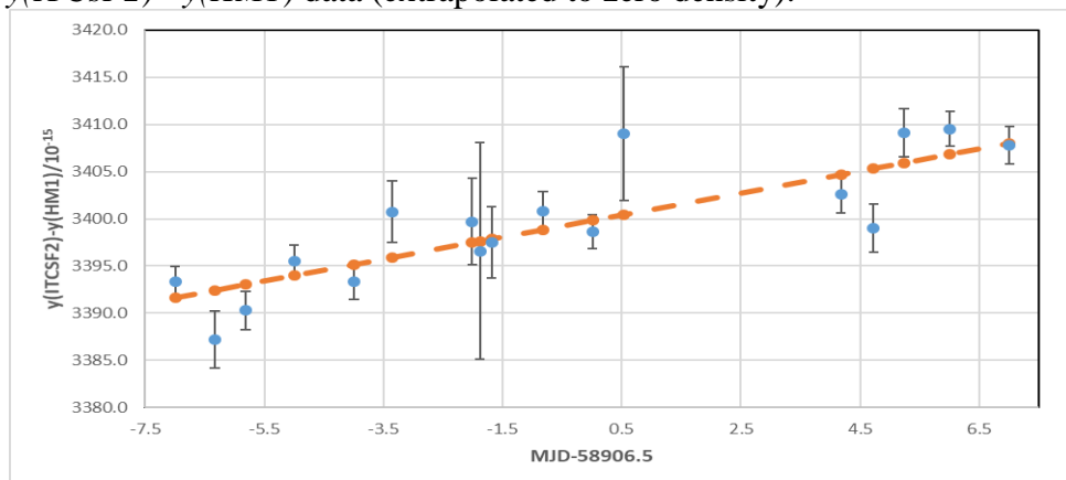
Figure 3. y(ITCsF2) - y(HM1) - data and the linear fit curve.
