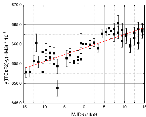
Figure 3. y(ITCsF2) - y(HM3) - data and the linear fit curve.
