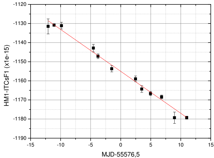
Figure 3. y(HM1) - y(IT-CsF1) data (biases corrected) and the linear fit curve (straight line).
