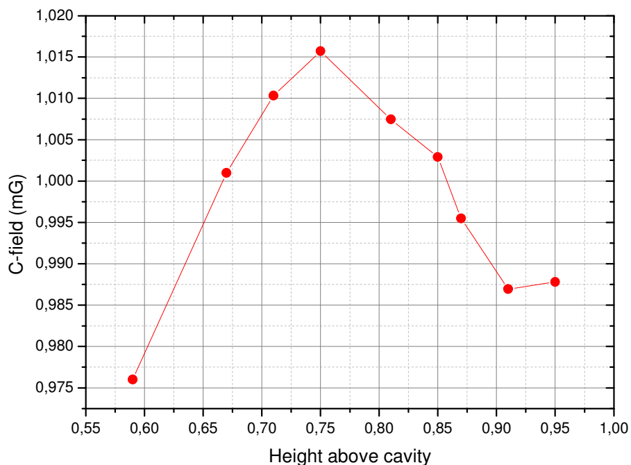
Figure 1. C-field map, January 2011.
